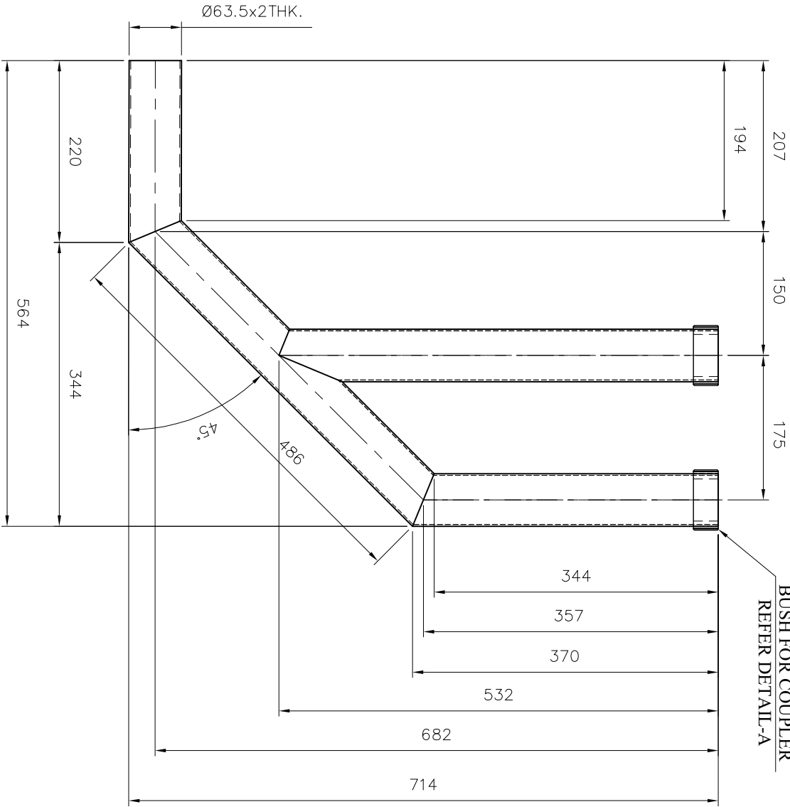
DETAIL OF BRANCH PIPE
